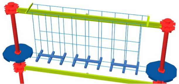
E105: Stirrup Rope Beam with Handlines
