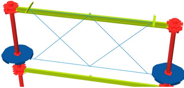
E86: Alternating Deep Burma Bridge with Handlines
